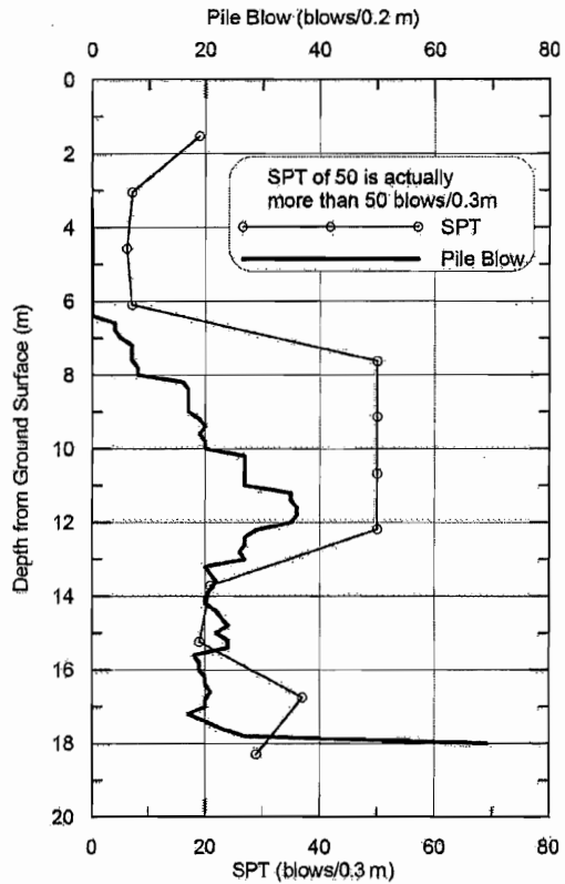
Figure 4. Example of Soft Clay Over Very Dense Sand Profile
