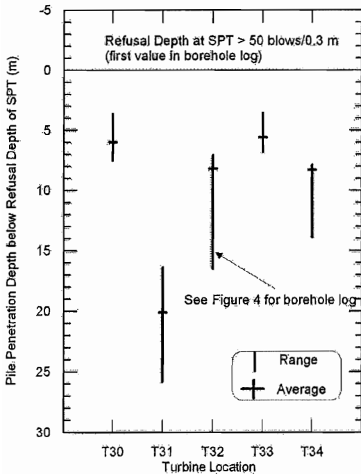
Figure 7. Actual Pile Depths vs Refusal Depths of SPT
