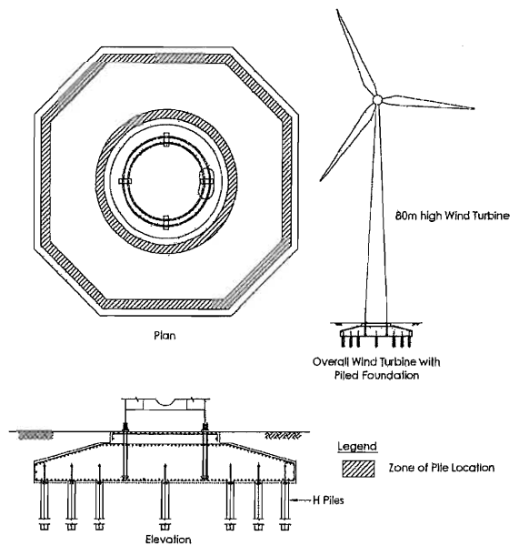
Figure 2. Piled Foundation for Wind Turbine
