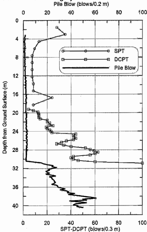
Figure 3. Typical Soft Clay Profile
