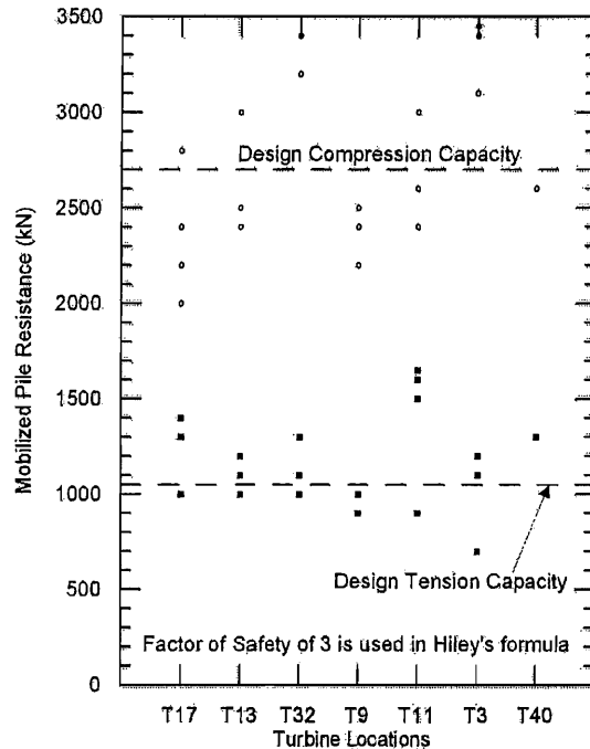
Figure 5. Mobilized Pile Resistance from PDA Tests
