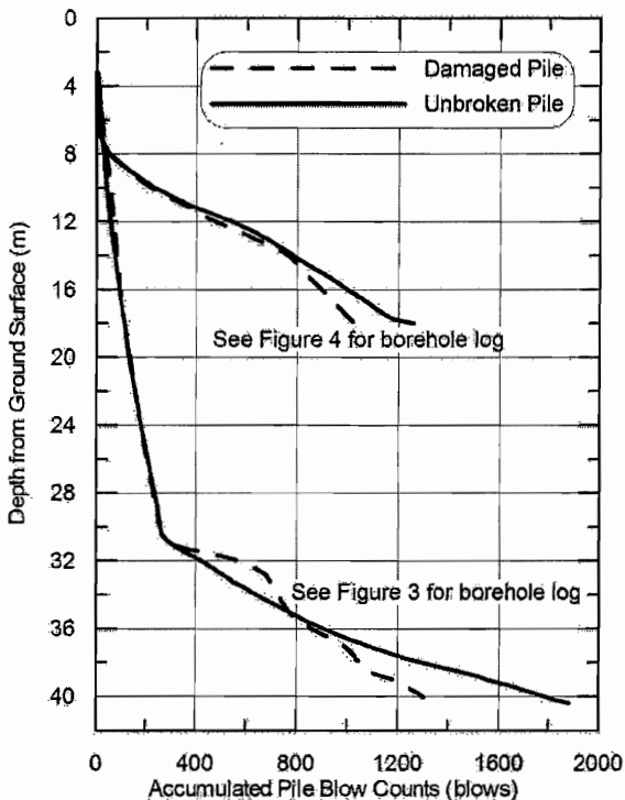
Figure 9 Accumulated Pile Blow Counts
