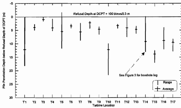
Figure 6. Actual Pile Depths vs Refusal Depths of DCPT
